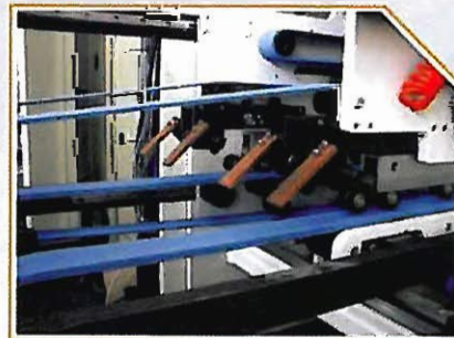
Stopper at trombone section to align leading edge feeding into compression section
