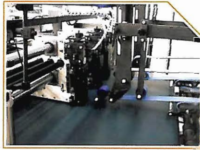
Stopper / Presser at entrance of compression belt to prevent fishtailing
